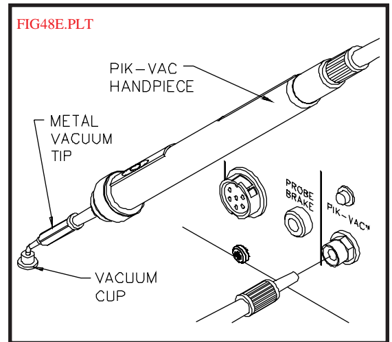
Figure 109. Pik-Vac Set-Up
