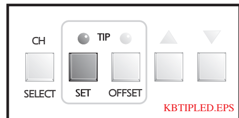
Figure 86. Press Tip Set Key
