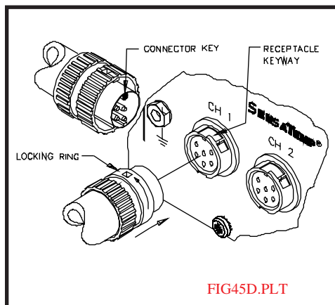
Figure 17. TMC Handpiece Connection
