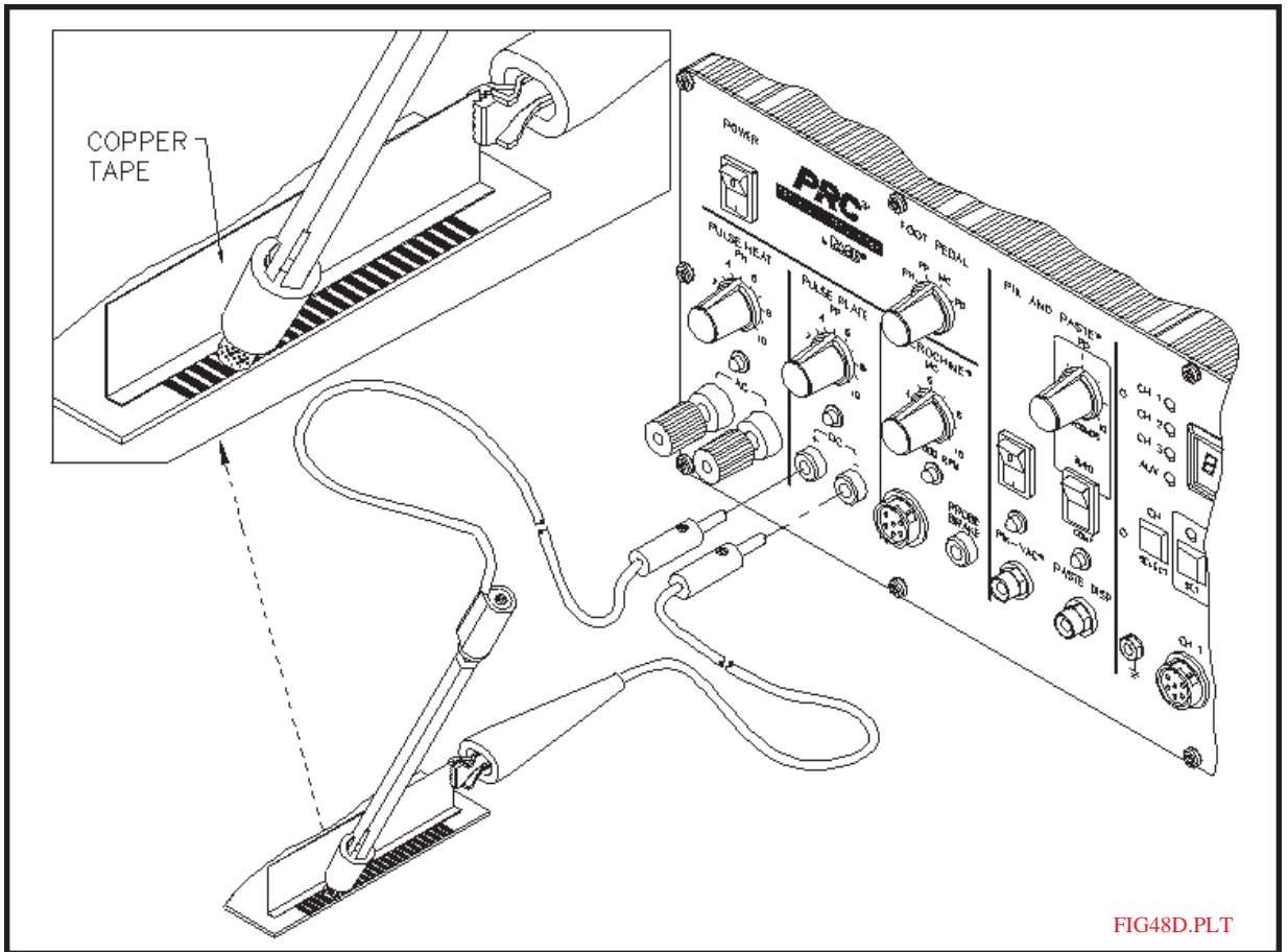
Figure 122. Pulse Plate Set-Up
