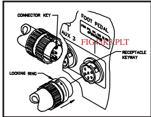
Figure 97. Foot Pedal Connection
