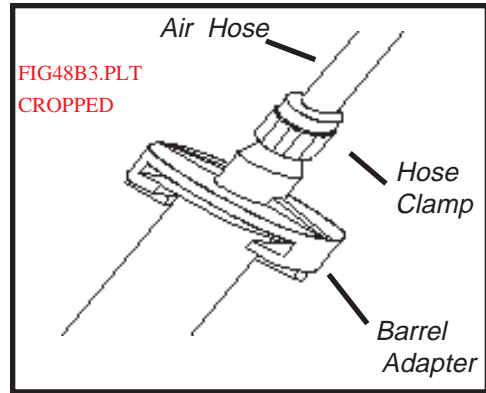
Figure 103. Barrel Adapter Connect.
