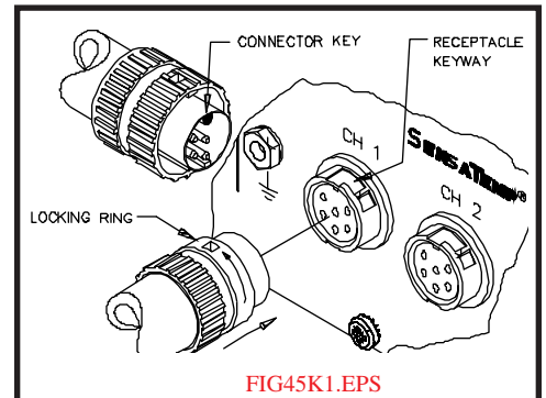
Figure 27. Handpiece Connection, TMC
