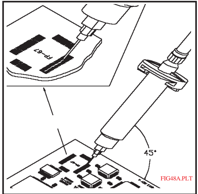
Figure 107. Paste Dispensing
