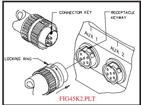
Figure 35. Aux. Accessory Connection
