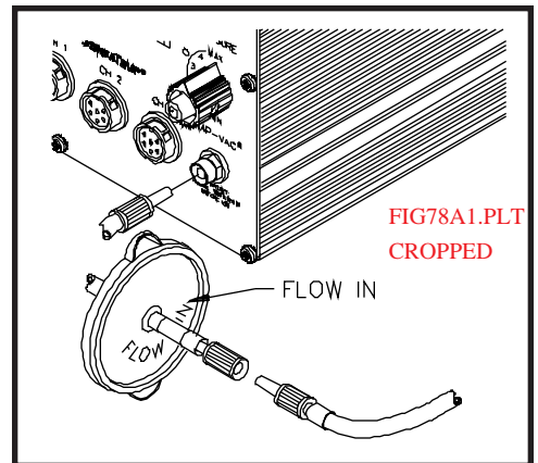
Figure 22. VisiFilter Preparation
